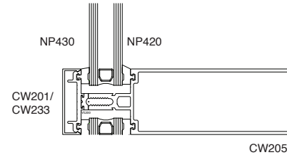
② SILL
