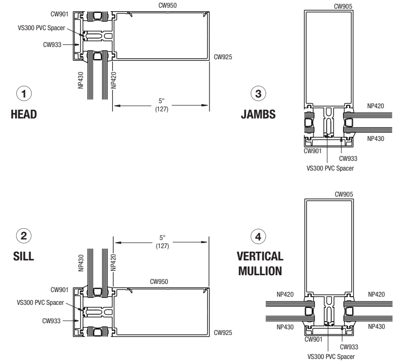
TYPICAL DETAILS:
