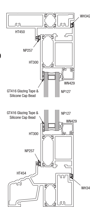
1 HEAD
