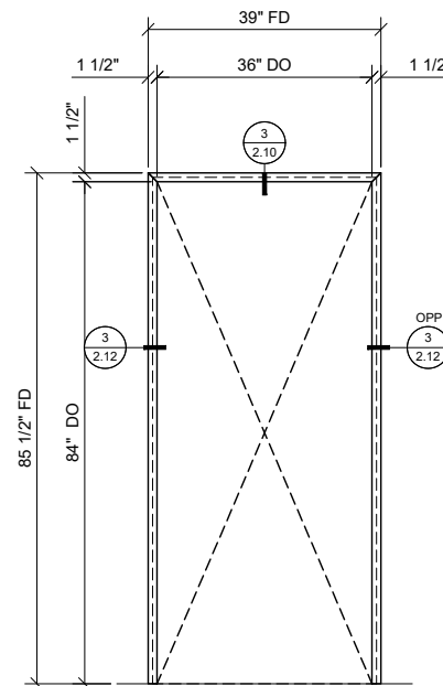
3 ELEVATION: SINGLE CASED OPENING 3/4" = 1'-0" ARCH. REF.: N/A
