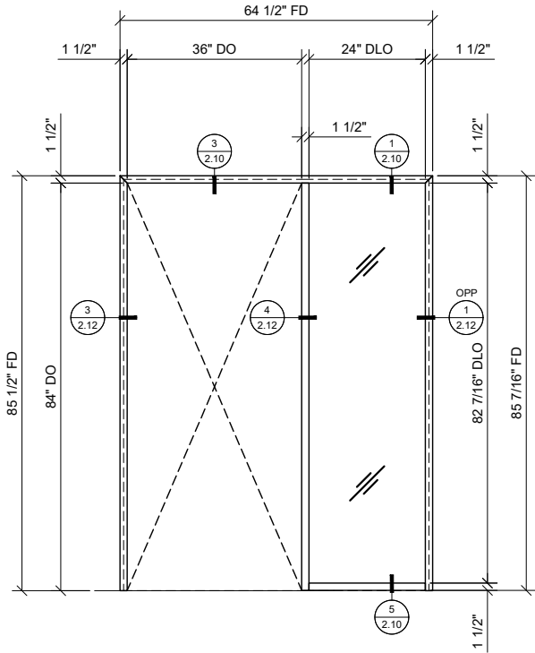
1 ELEVATION: SINGLE CASED OPENING WITH FULL HEIGHT SIDELITE 3/4" = 1'-0" ARCH. REF.: N/A
