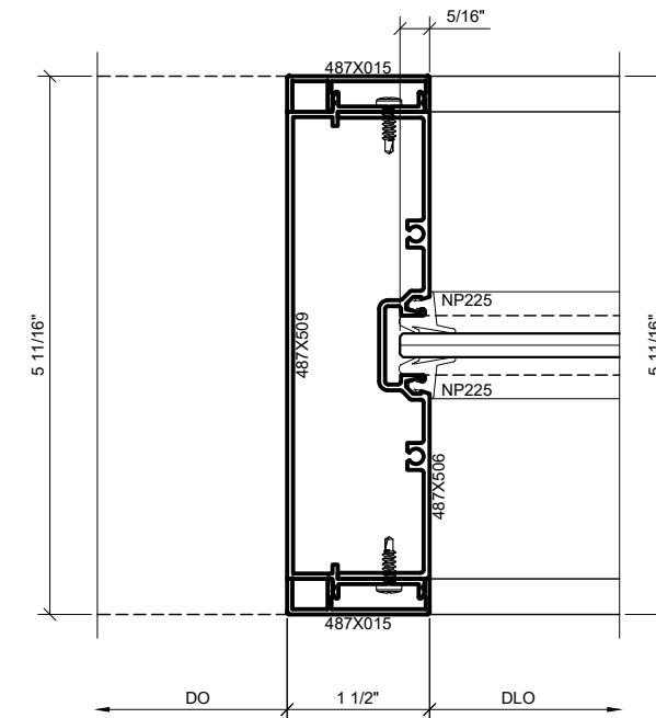
④ CASSED OPENING JAMB DETAIL AT SIDELITE 1'-0" = 1'-0" ARCH. REF.: N/A
