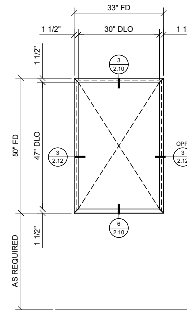
4 ELEVATION: SINGLE CASED PASS-THRU 3/4" = 1'-0" ARCH. REF.: N/A
