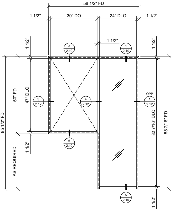
2 ELEVATION: SINGLE CASED OPENING ABOVE FLOOR WITH FULL HEIGHT SIDELITE 3/4" = 1'-0" ARCH. REF.: N/A
