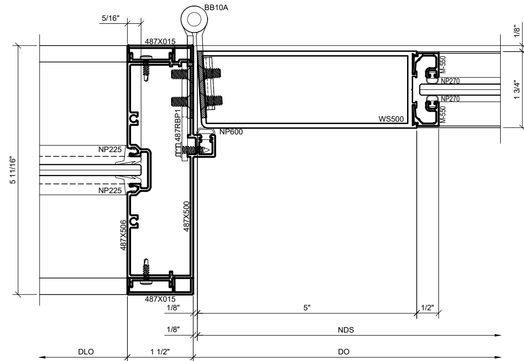
① DOOR JAMB DETAIL AT HINGE SIDE WITH SIDELITE W/ SERIES 550 WIDE STILE DOOR 1'-0" = 1'-0" ARCH. REF.: N/A
