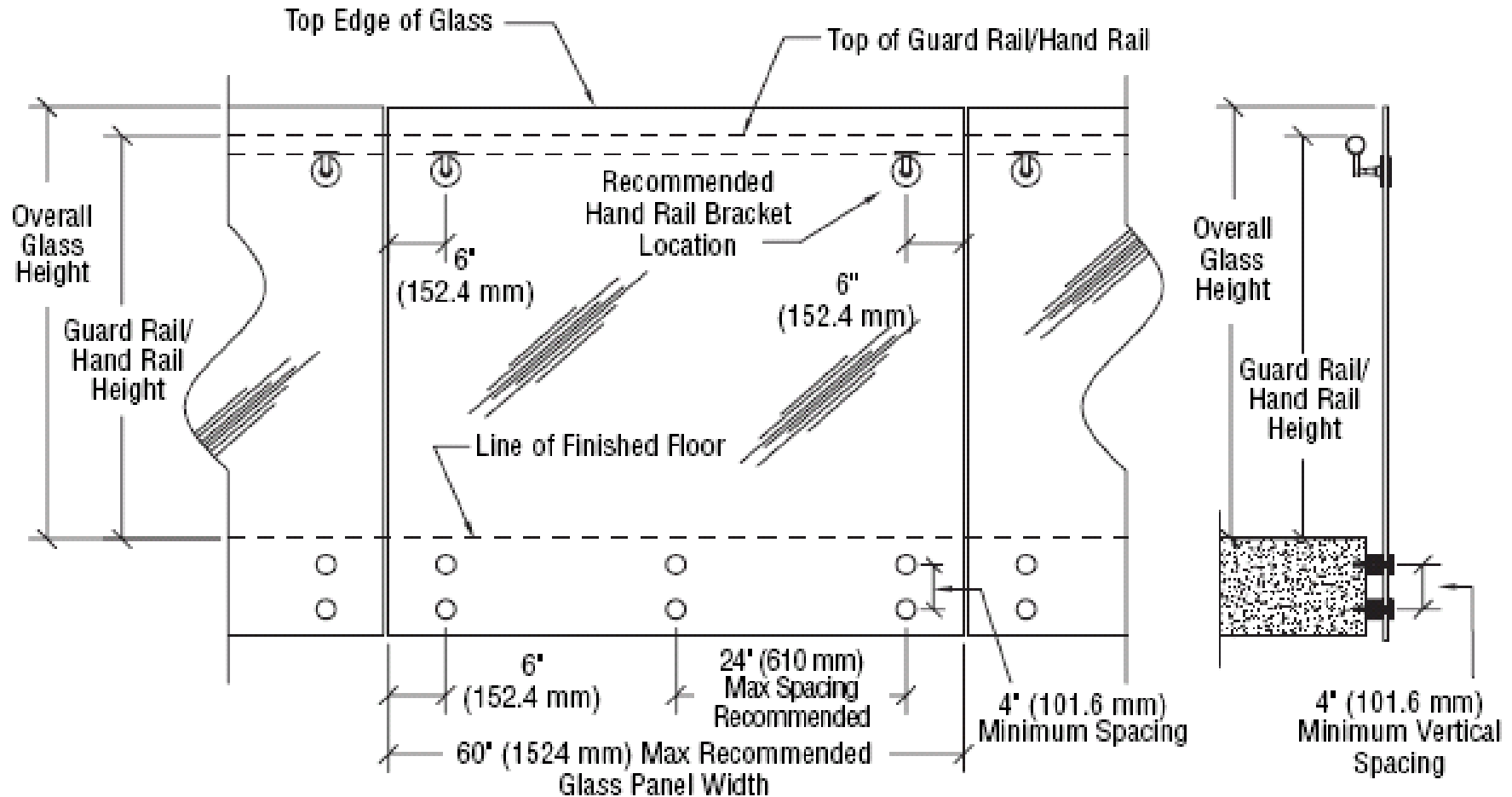
Typical Standoff Glass Rail Elevation
